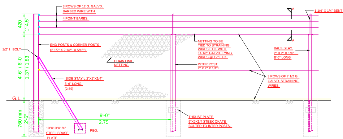
CHAIN LINK FENCING
