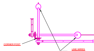
METHOD OF SECURING LINE WIRES TO POSTS
