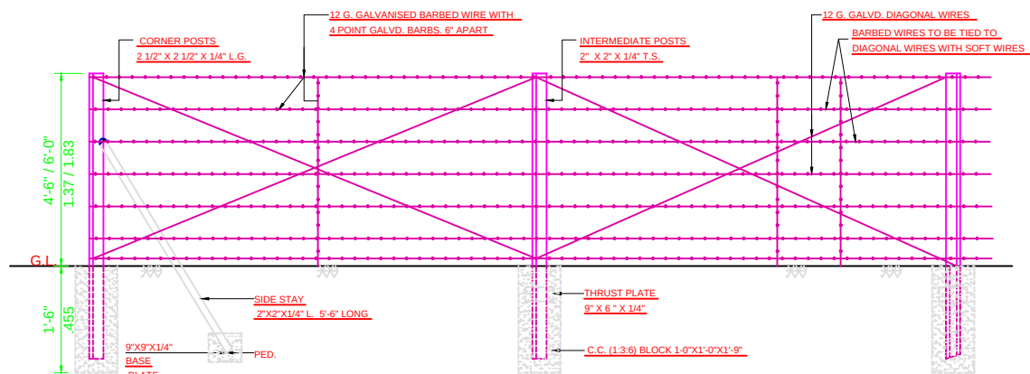
BARBED WIRE FENCING
