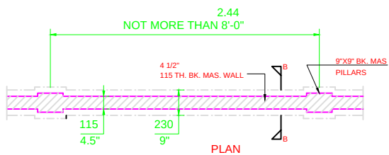
BRICK MASONRY COMPOUND WALL
